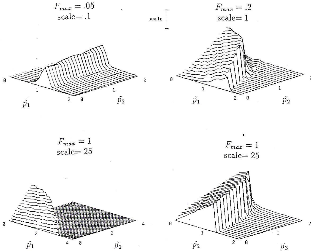
Fig. 1 illustrates the final energy E(T = 50) = .5\dot{y}^2 + V(y, \vec{p}) versus the parameters of the model of the potential V(x, \vec{p}) = .5\tilde{p}_1 x^2 + .25\tilde{p}_2 x^4 + .01\tilde{p}_3 x^6 , where p_1 = p_2 = p_3 = 1 are the parameters of the experimental system and where the magnitude of the driving force has various values. The initial conditions are y = \dot{y} = 0 and x = \dot{x} \approx .02 . At resonance, i.e. for \tilde{p}_1 = \tilde{p}_2 = \tilde{p}_3 = 1 the final energy is more than one order of magnitude larger than the largest final energy due to a sinusoidal perturbation with the same amplitude ( F_{max} = 1 ).
