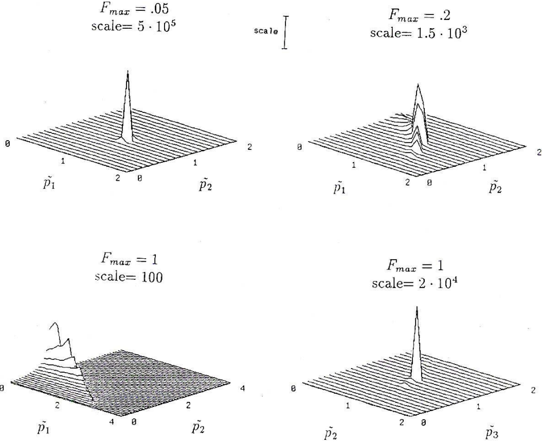
Fig. 2 illustrates the ratio between the transferred and the reflected energy versus the parameters of the model of the potential V(x, \vec{p}) = .5\tilde{p}_1 x^2 + .25\tilde{p}_2 x^4 + .01\tilde{p}_3 x^6 , where p_1 = p_2 = p_3 = 1 are the parameters of the experimental system and where the magnitude of the driving force has various values. The initial conditions are y = \dot{y} = 0 and x = \dot{x} \approx .02 .
